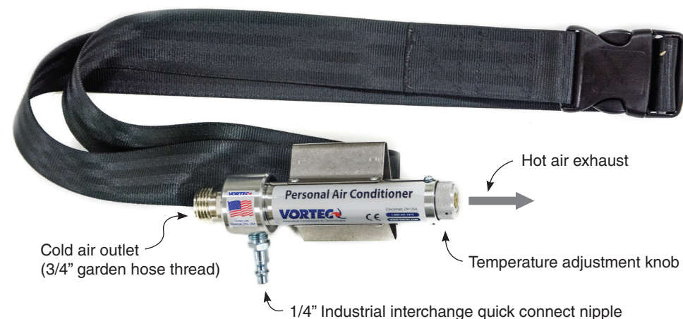
Figure 1. Personal Air Conditioner with belt installed for horizontal orientation
