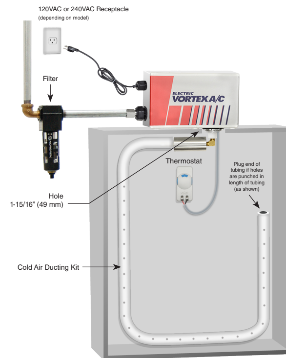
ELECTRIC VORTEX A/C TYPE 4/4X (SHOWN TOP MOUNTED ON CUSTOMER'S ENCLOSURE)
